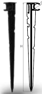
DAMLAMA BORU SABİTLEME KAZIĞI-UZUN DRIPLINE PIPE STAKE-LONG
