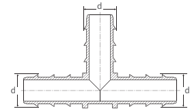
KURTAĞZI TE BARBED TEE
