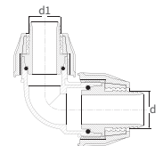
REDÜKSİYON DİRSEK REDUCING ELBOW
