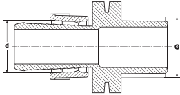
YÜZÜKLÜ YASSI - ERKEK NİPEL DRIP TAPE (WITH RING) - MALE NIPPLE
