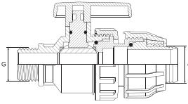
RURAL KÜRESEL VANA ERKEK - KABLİN RURAL BALL VALVE MALE - COUPLING
