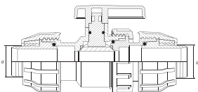
RURAL KÜRESEL VANA KABLİN - KABLİN RURAL BALL VALVE COUPLING - COUPLING
