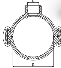
PRİZ KOLYE GEÇMELİ CLAMP SADDLE WITH SLIDE
