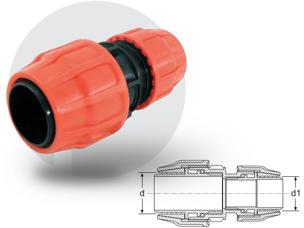
LAYFLAT REDÜKSİYON MANŞON LAYFLAT REDUCING COUPLING
