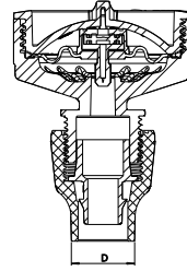
HAT SONU TAHLİYE VANASI - KİLİTLİ BAĞLANTI AUTOMATIC LINE FLUSH VALVE – LOCK TYPE
