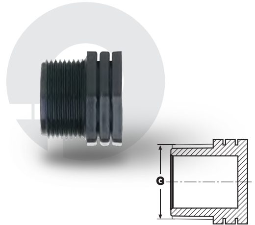
DİŞLİ KÖR TAPA ERKEK THREADED END CAP MALE
